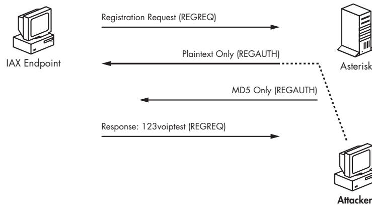
Figure 5-9: Downgrade attack
